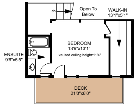
UPPER FLOOR 403 SQ.FT
